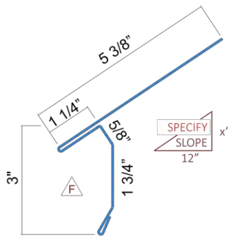
Steep Slope Extended Eave, 3" Face For slopes up to 12:12
