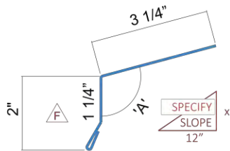
Eave Drip Edge, 2" Face For all slopes
