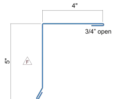
Box Gable Trim, 5" Face
